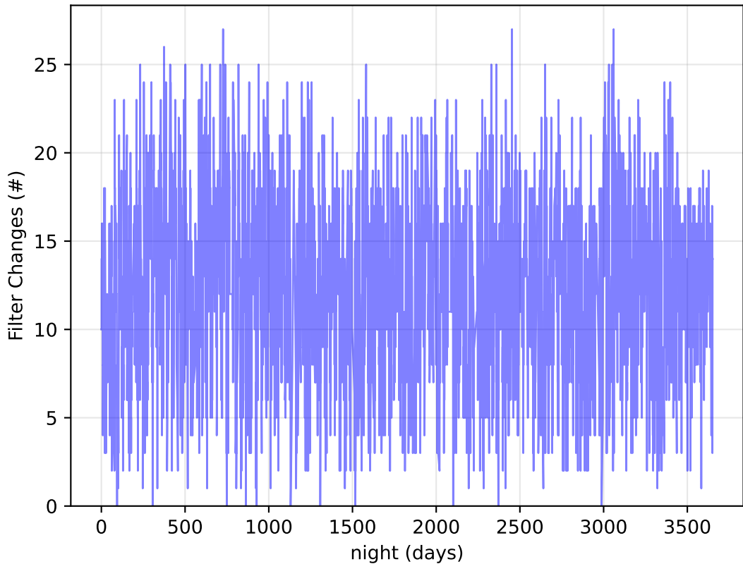
internal_u_expt30_nscale1.0v3.4_10yrs Per Night: Filter Changes
