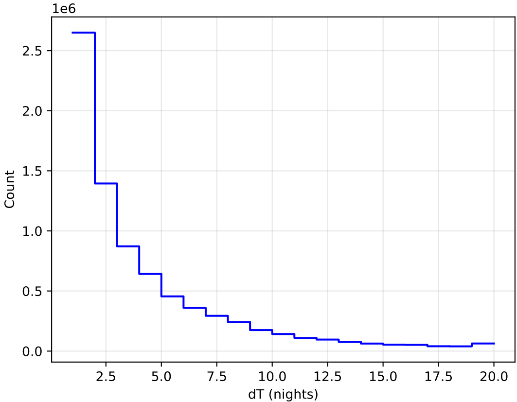
internal_u_expt30_nscale1.0v3.4_10yrs WFD all bands: DeltaNight Histogram
