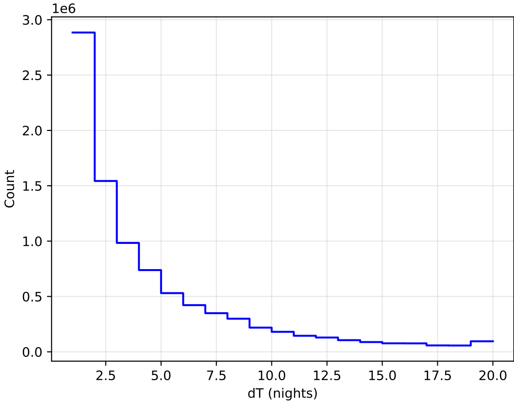
internal_u_expt30_nscale1.0v3.4_10yrs All sky all bands: DeltaNight Histogram
