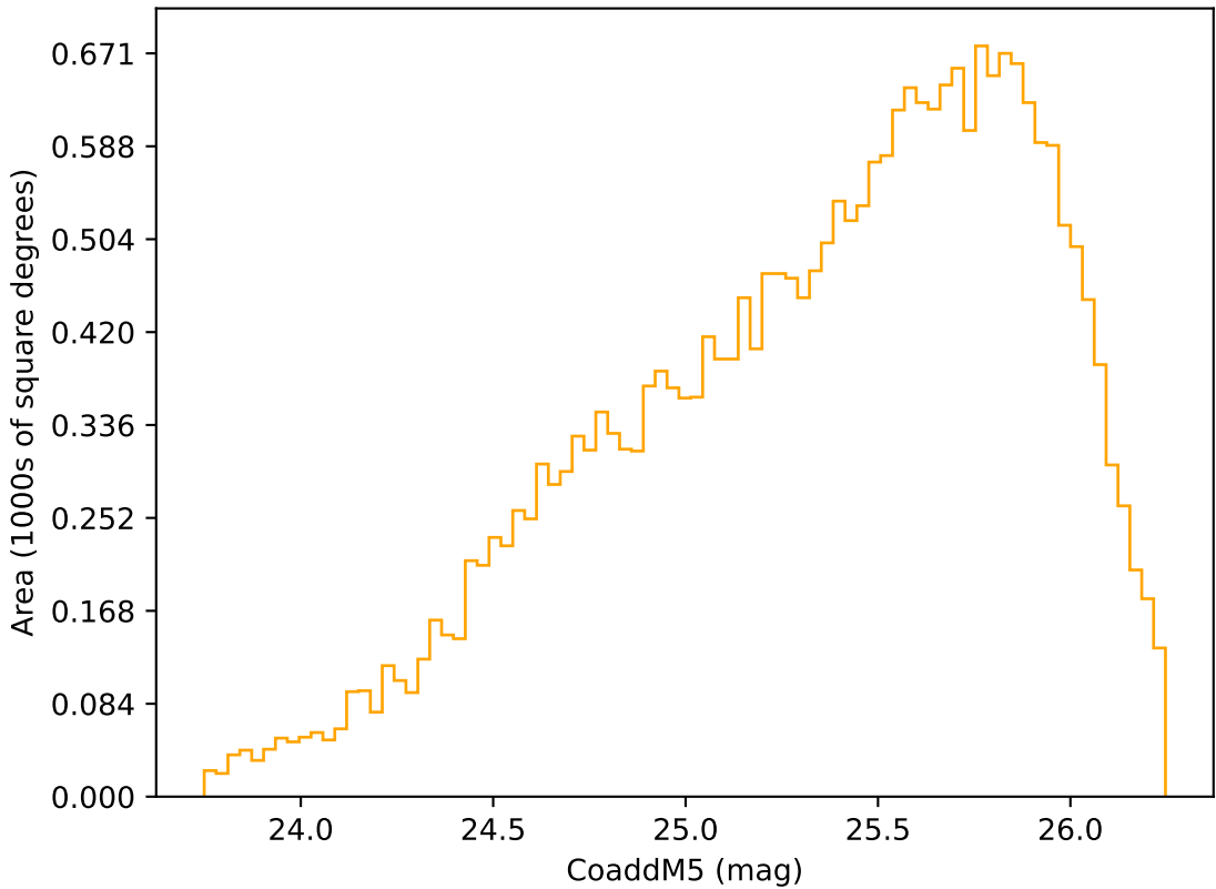
internal_u_expt30_nscale1.0v3.4_10yrs Yr 3-4 r band: CoaddM5
