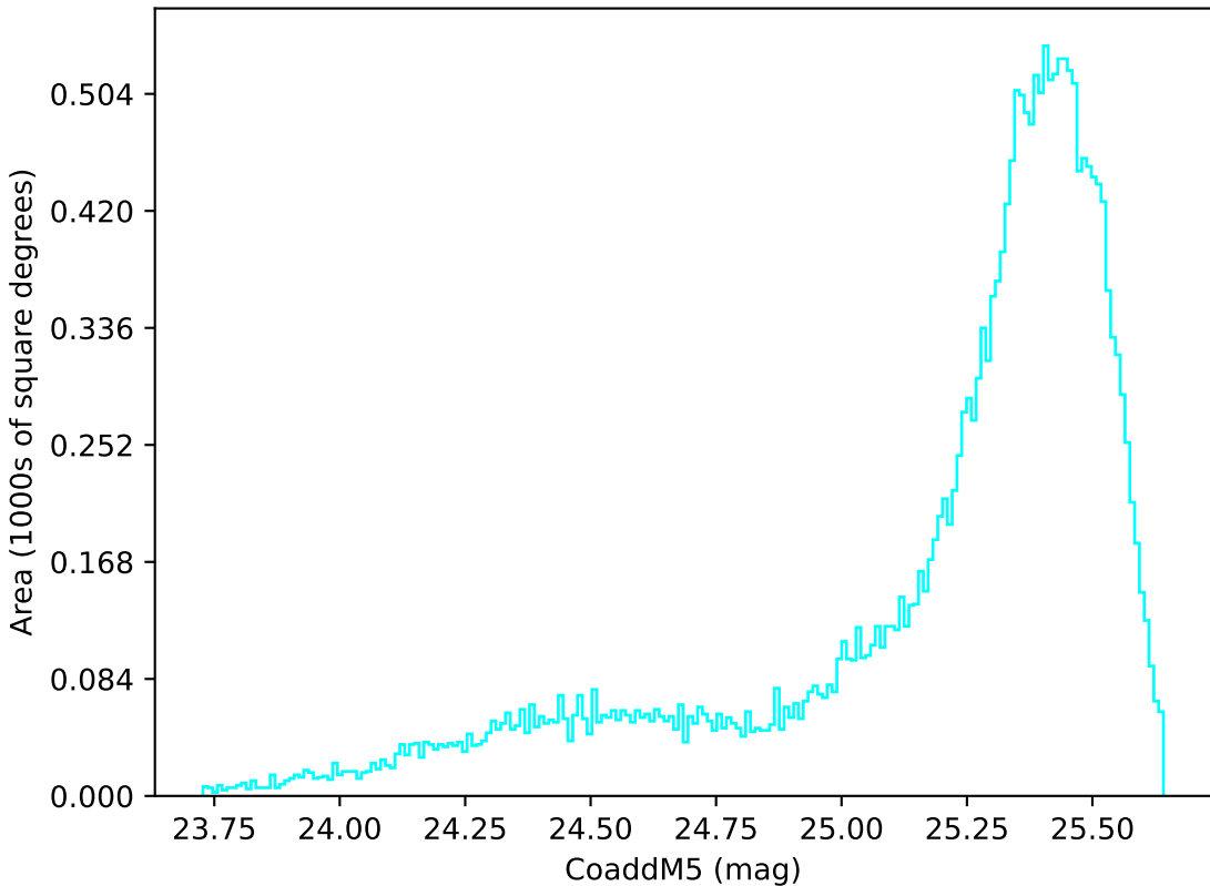
internal_u_expt30_nscale1.0v3.4_10yrs All sky u band: CoaddM5
