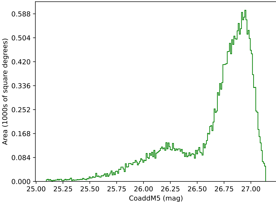
internal_u_expt30_nscale1.0v3.4_10yrs All sky g band: CoaddM5
