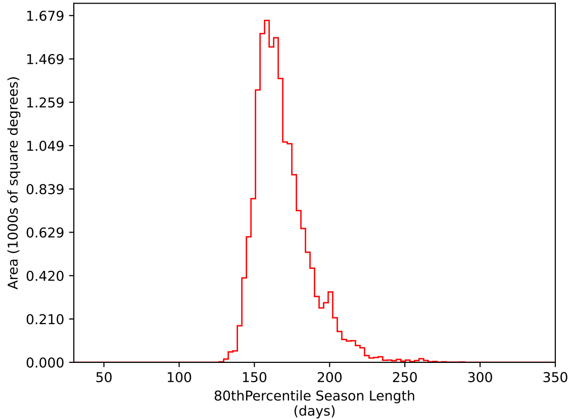
internal_u_expt30_nscale1.0v3.4_10yrs WFD i band: 80thPercentile Season Length
