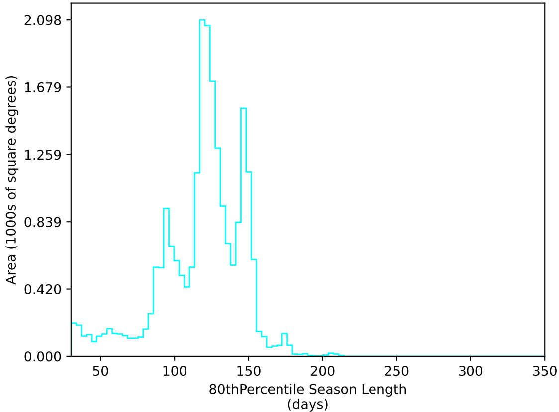
internal_u_expt30_nscale1.0v3.4_10yrs All sky u band: 80thPercentile Season Length
