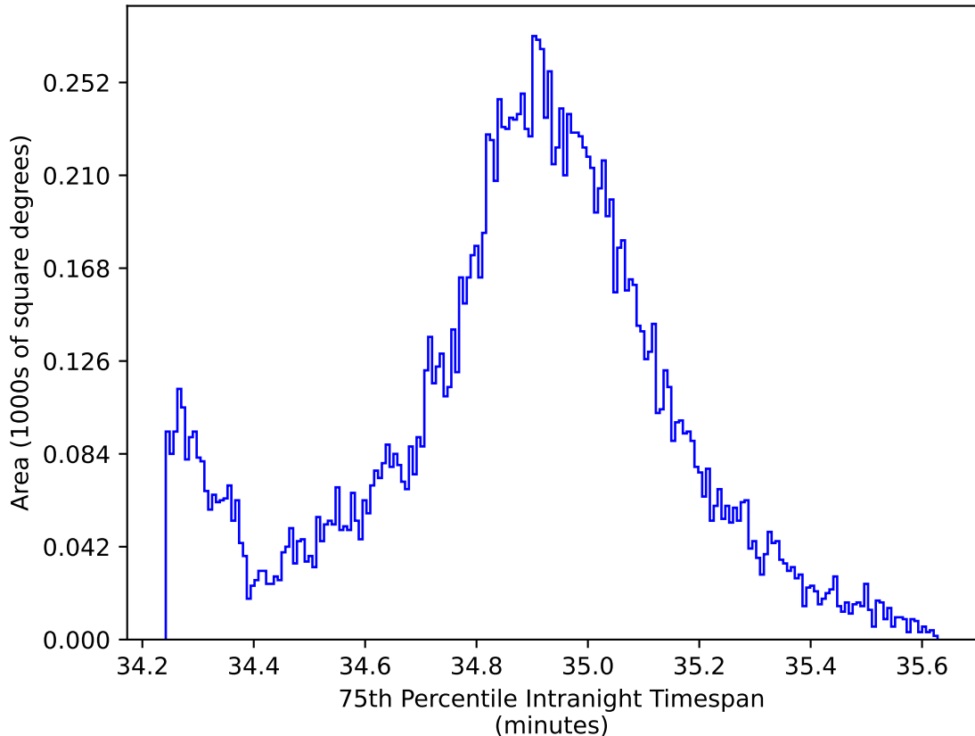
internal_u_expt30_nscale1.0v3.4_10yrs WFD all bands: 75th Percentile Intranight Timespan
