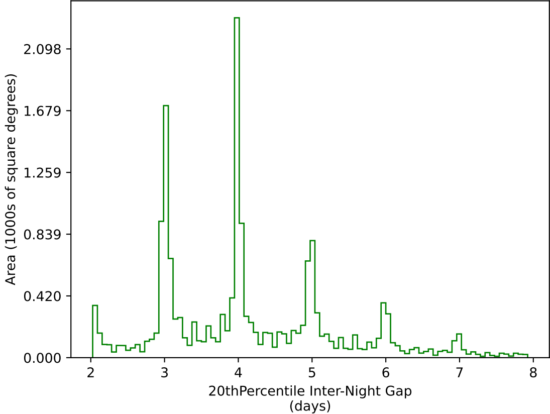
internal_u_expt30_nscale1.0v3.4_10yrs WFD g band: 20thPercentile Inter-Night Gap
