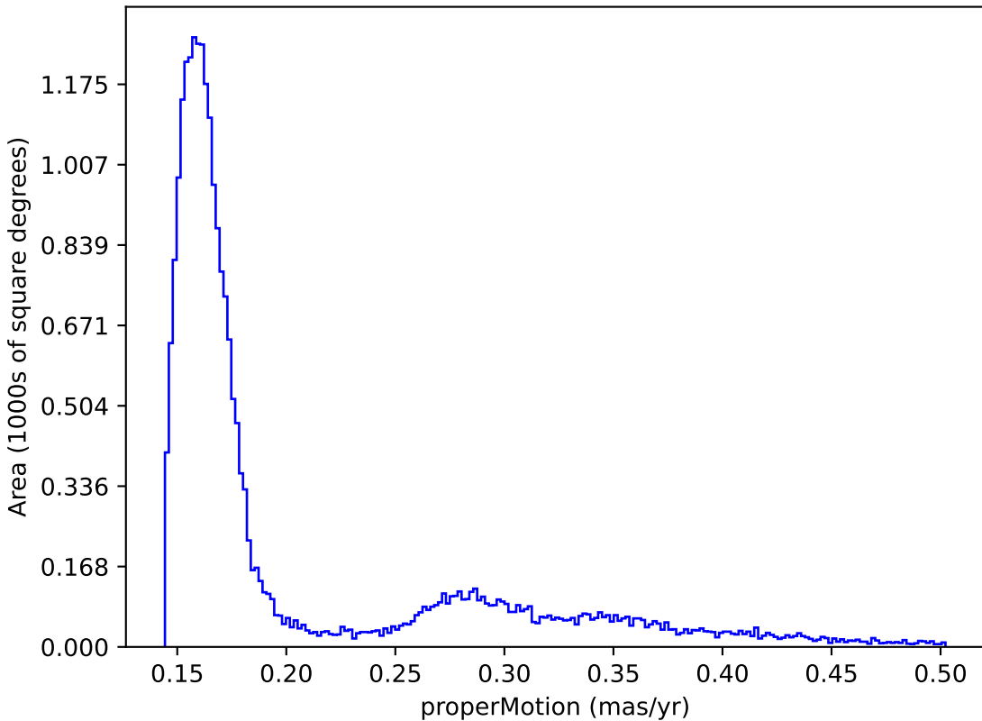
internal_u_expt30_nscale1.0v3.4_10yrs : properMotion
