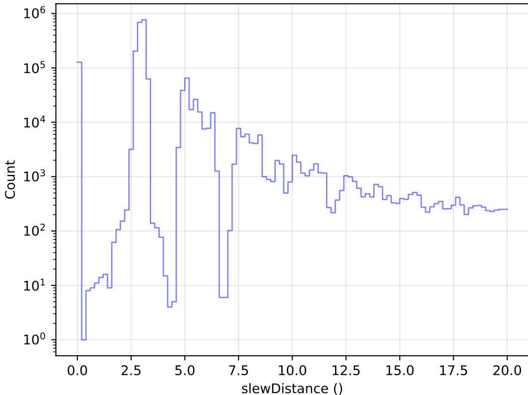
internal_u_expt30_nscale1.0v3.4_10yrs All visits: Zoom Slew Distance Histogram
