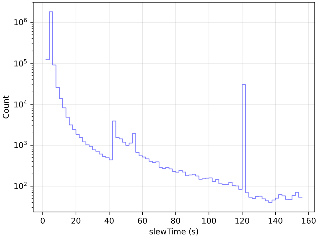
internal_u_expt30_nscale1.0v3.4_10yrs All visits: Slew Time Histogram
