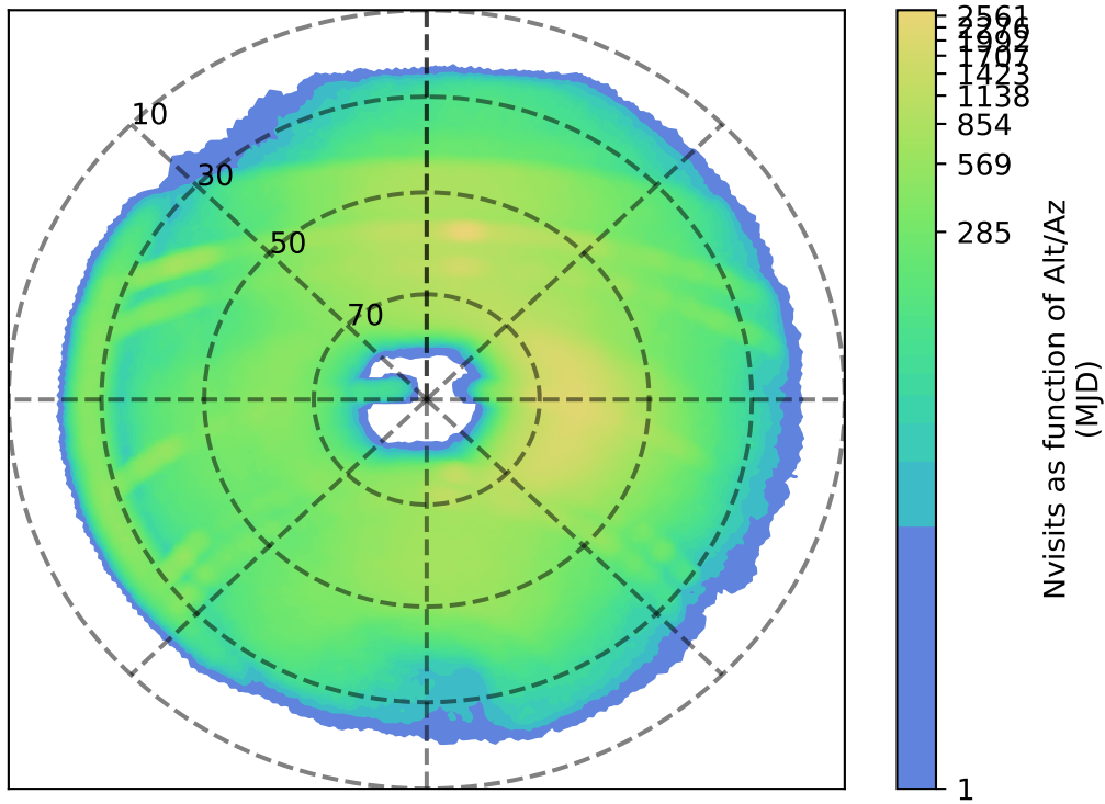
internal_u_expt30_nscale1.0v3.4_10yrs r: Nvisits as function of Alt/Az
