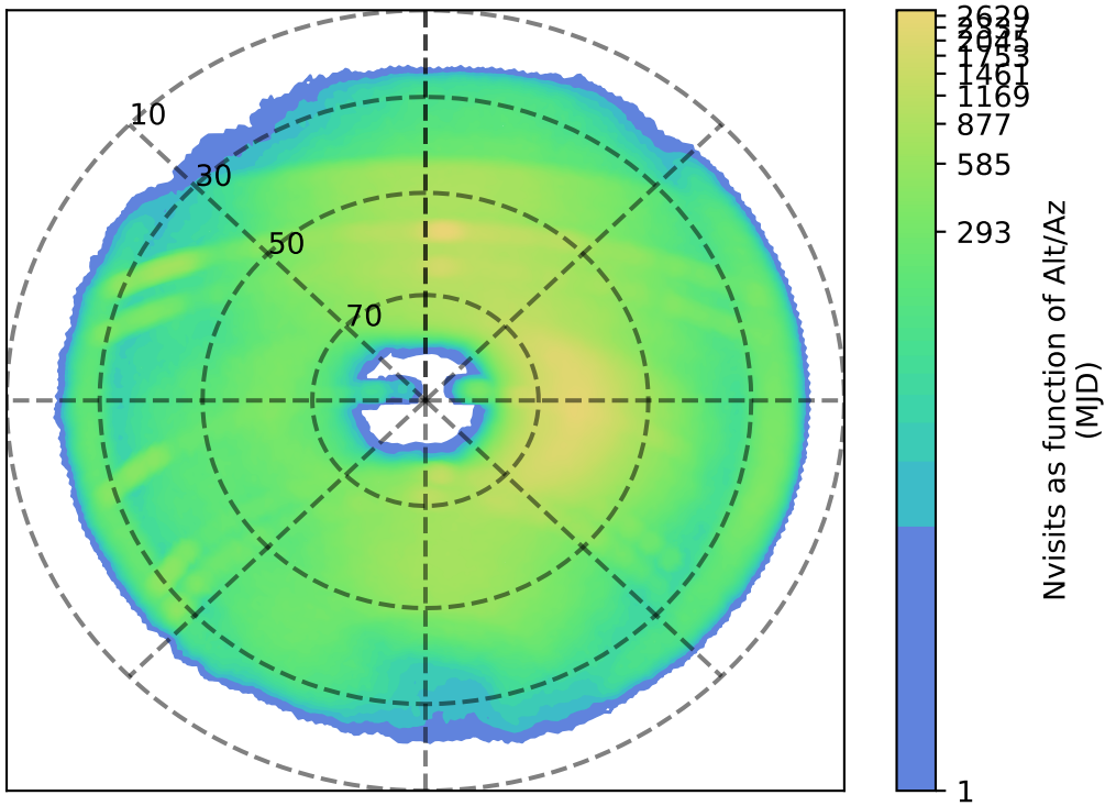
internal_u_expt30_nscale1.0v3.4_10yrs i: Nvisits as function of Alt/Az
