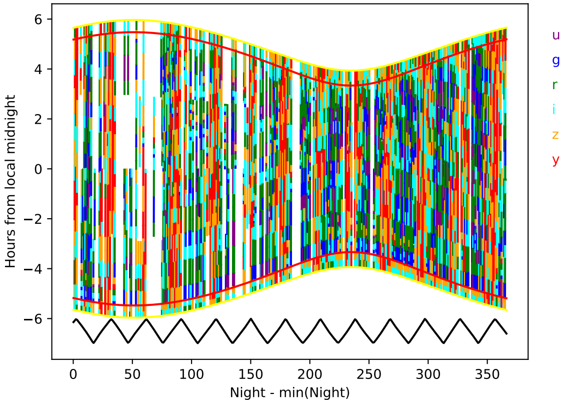
internal_u_expt30_nscale1.0v3.4_10yrs year 9-10: Hourglass
