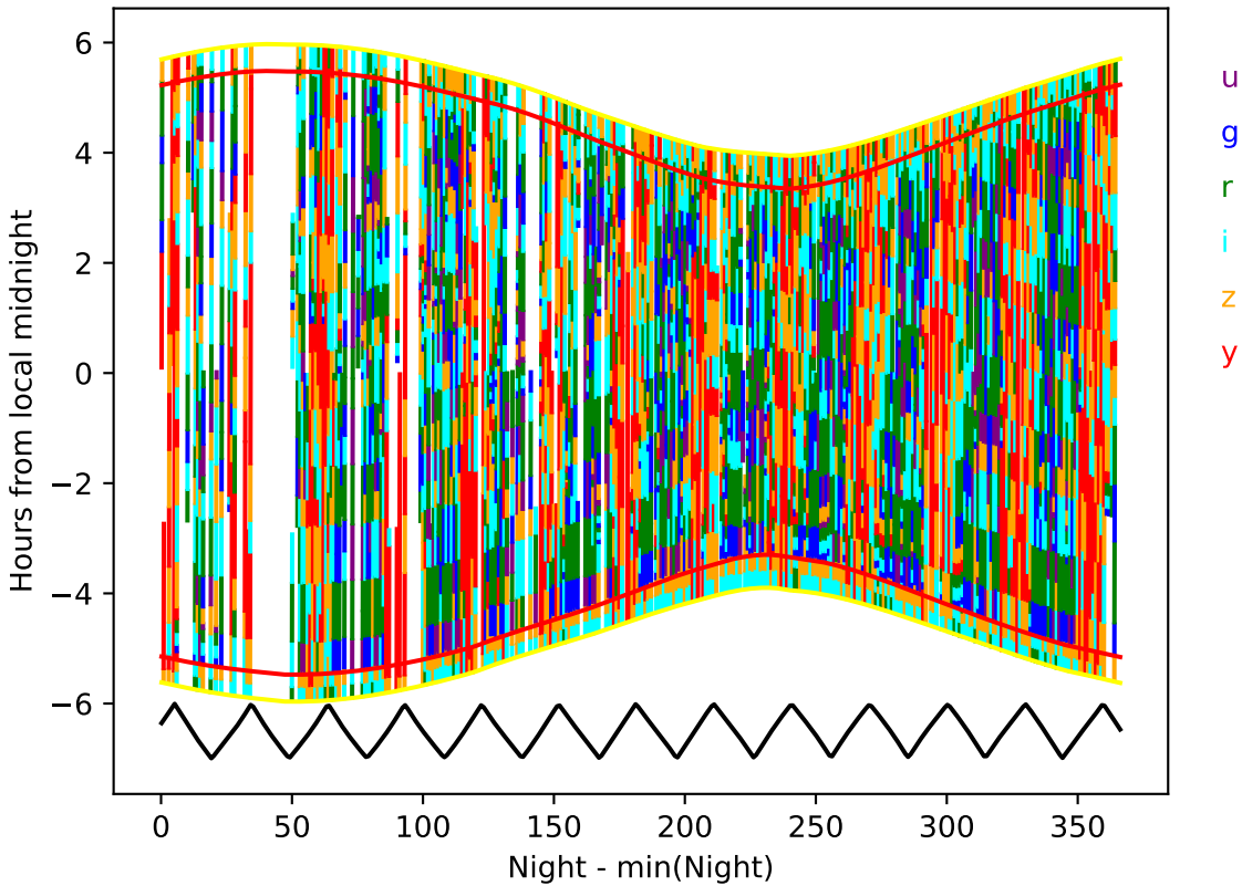
internal_u_expt30_nscale1.0v3.4_10yrs year 6-7: Hourglass
