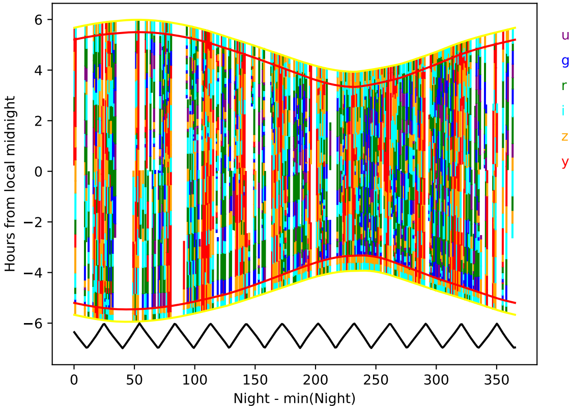
internal_u_expt30_nscale1.0v3.4_10yrs year 4-5: Hourglass
