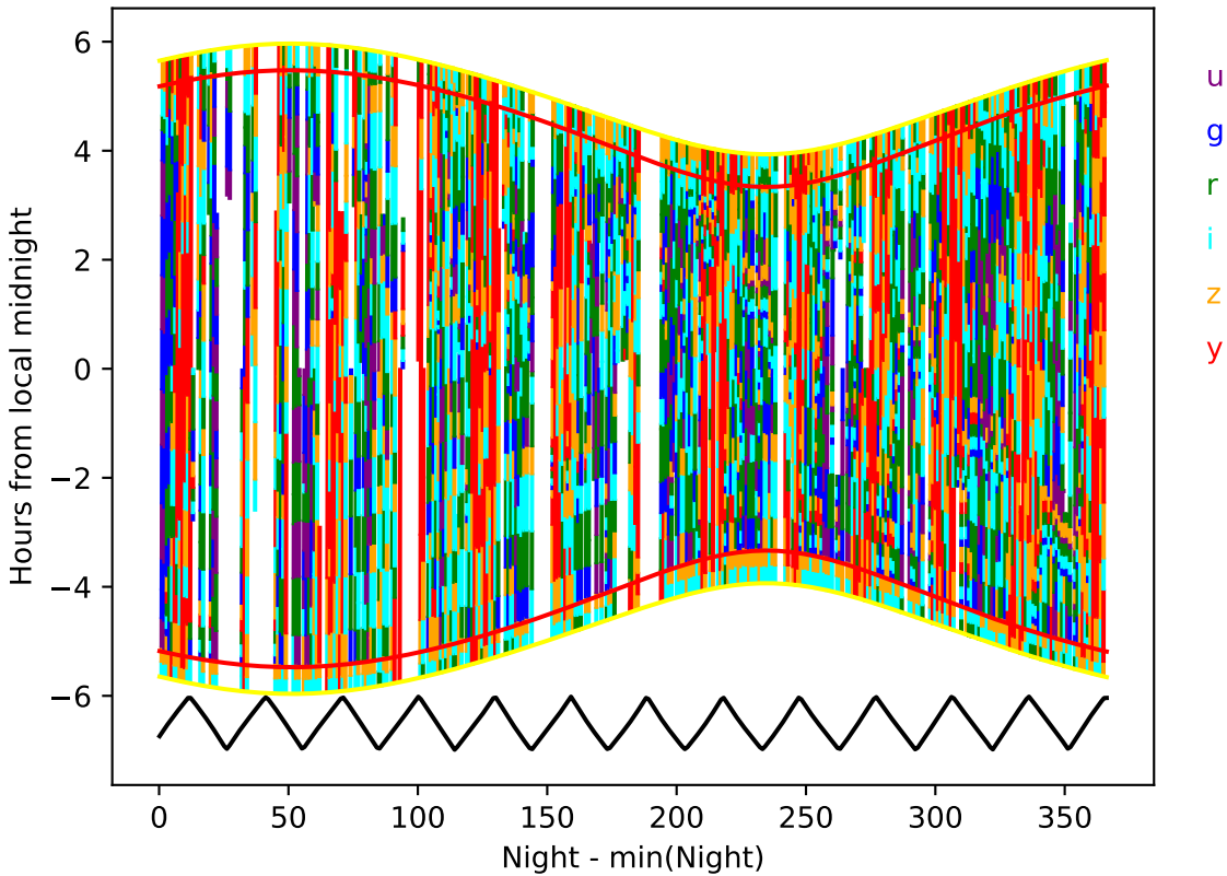
internal_u_expt30_nscale1.0v3.4_10yrs year 0-1: Hourglass
