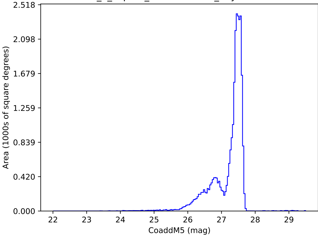
internal_u_expt30_nscale1.0v3.4_10yrs : CoaddM5
