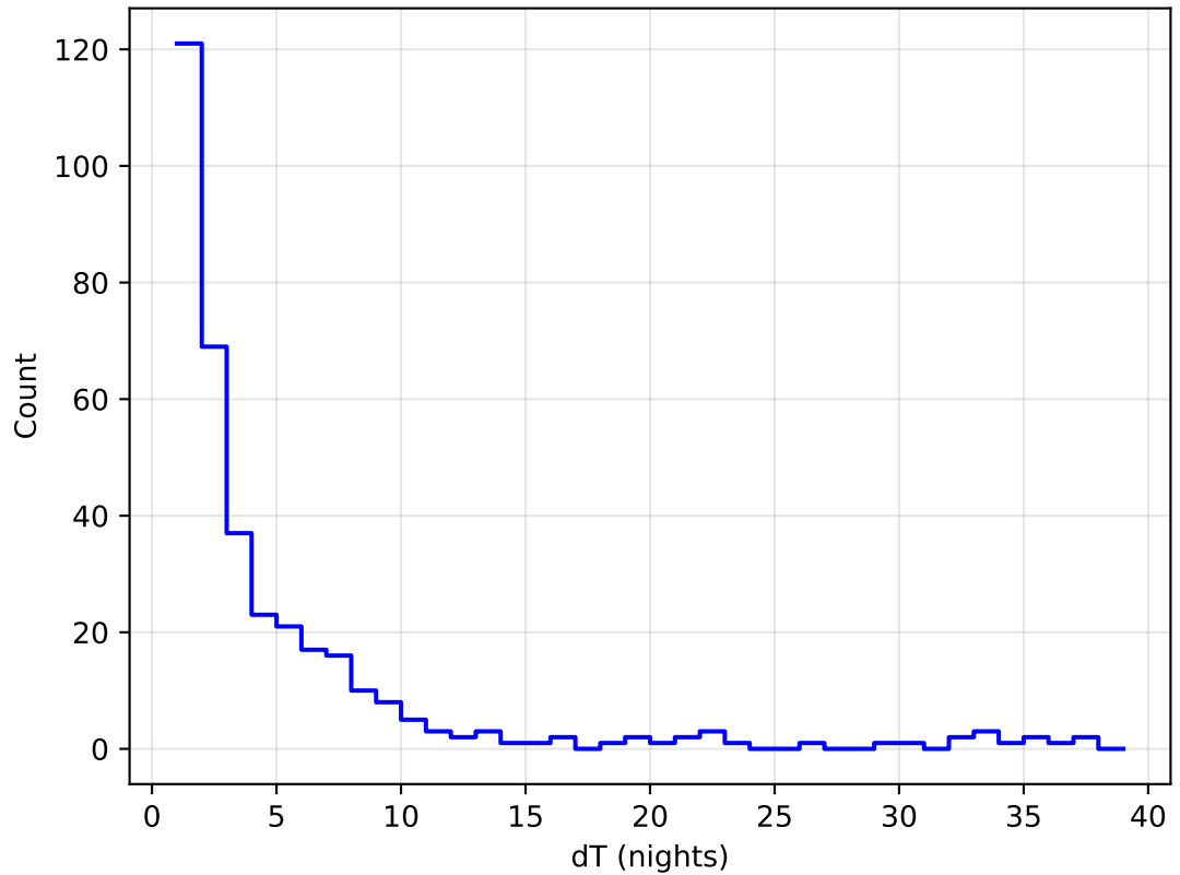
internal_u_expt30_nscale1.0v3.4_10yrs all bands: DD:WFD Delta Nights Histogram
