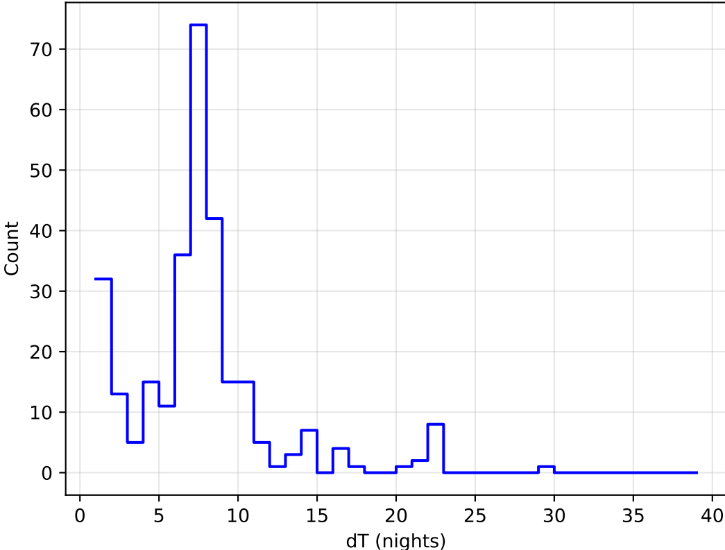
internal_u_expt30_nscale1.0v3.4_10yrs all bands: DD:EDFS Delta Nights Histogram
