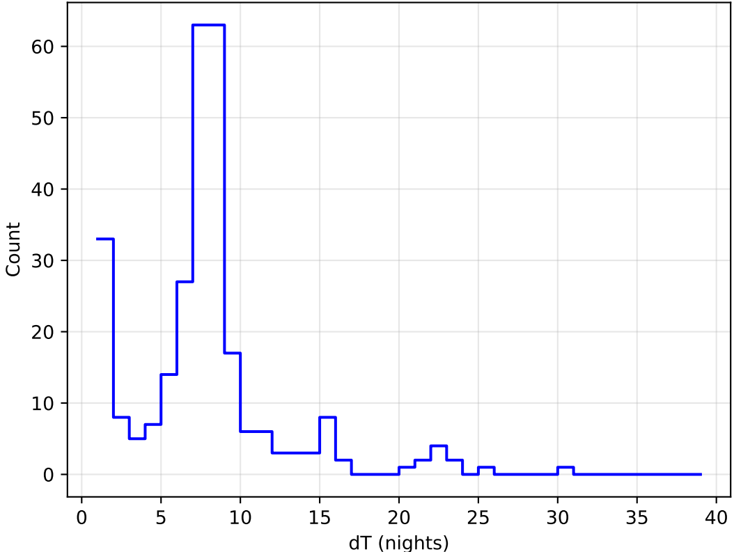
internal_u_expt30_nscale1.0v3.4_10yrs all bands: DD:ECDFS Delta Nights Histogram
