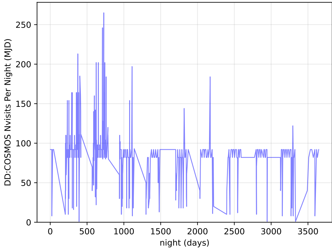
internal_u_expt30_nscale1.0v3.4_10yrs all bands: DD:COSMOS Nvisits Per Night
