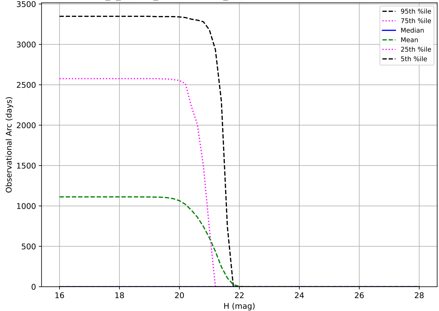
internal_u_expt30_nscale0.9v3.4_10yrs: Observational Arc Length Vatra
