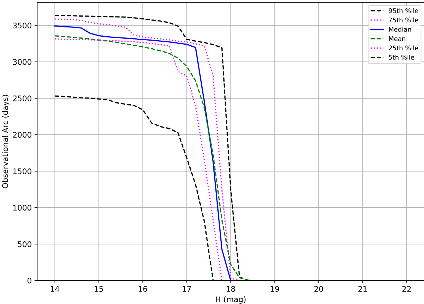
internal_u_expt30_nscale0.9v3.4_10yrs: Observational Arc Length Trojan
