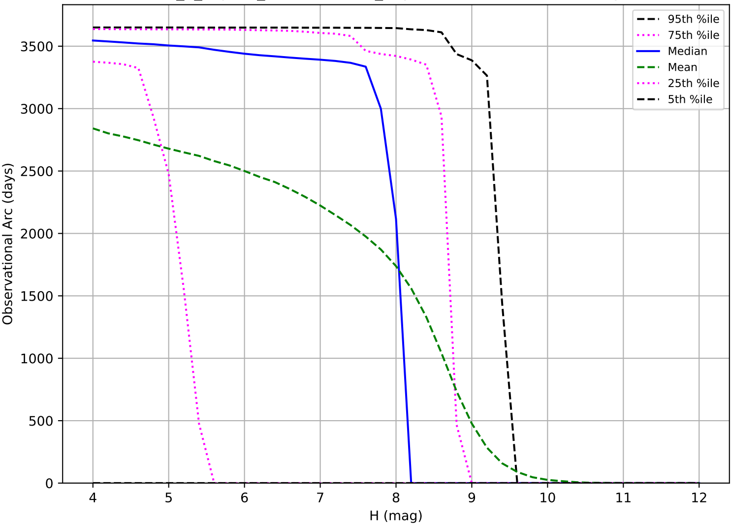
internal_u_expt30_nscale0.9v3.4_10yrs: Observational Arc Length TNO
