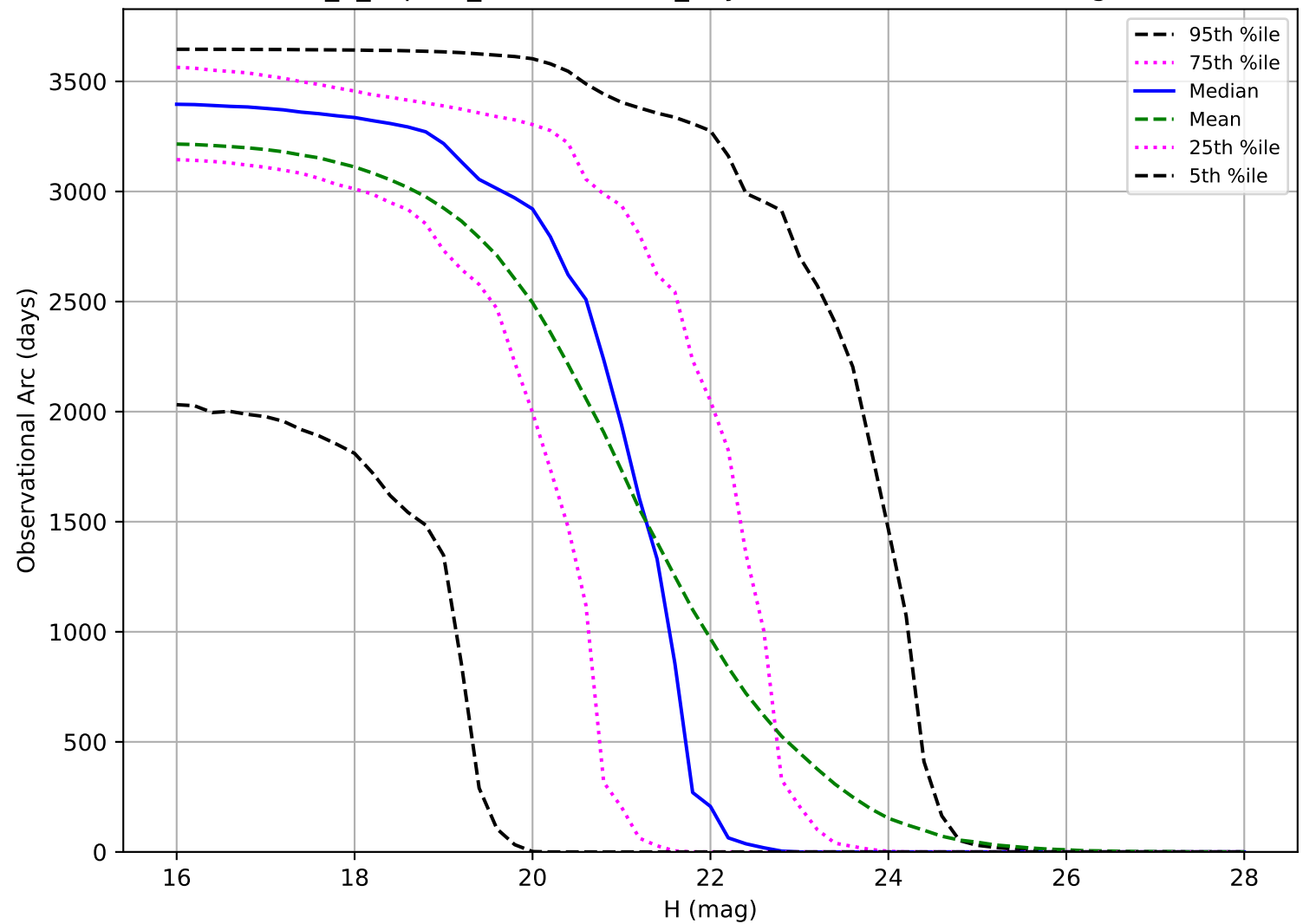
internal_u_expt30_nscale0.9v3.4_10yrs: Observational Arc Length PHA
