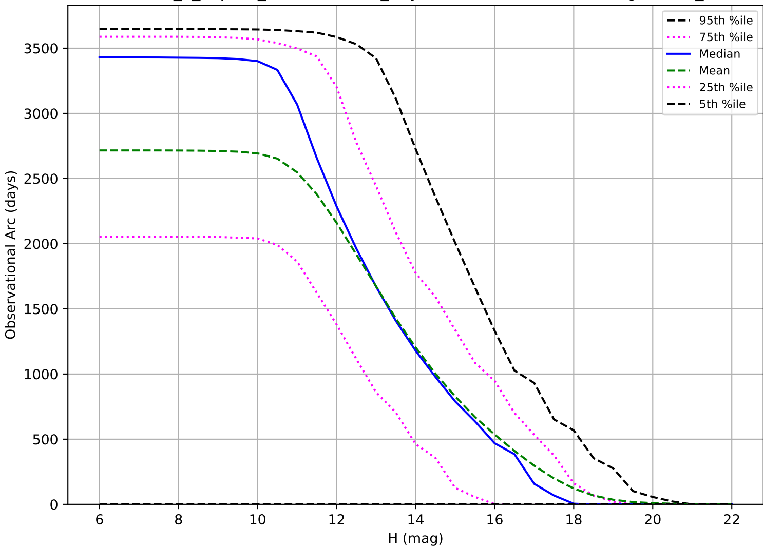
internal_u_expt30_nscale0.9v3.4_10yrs: Observational Arc Length OCC_r5
