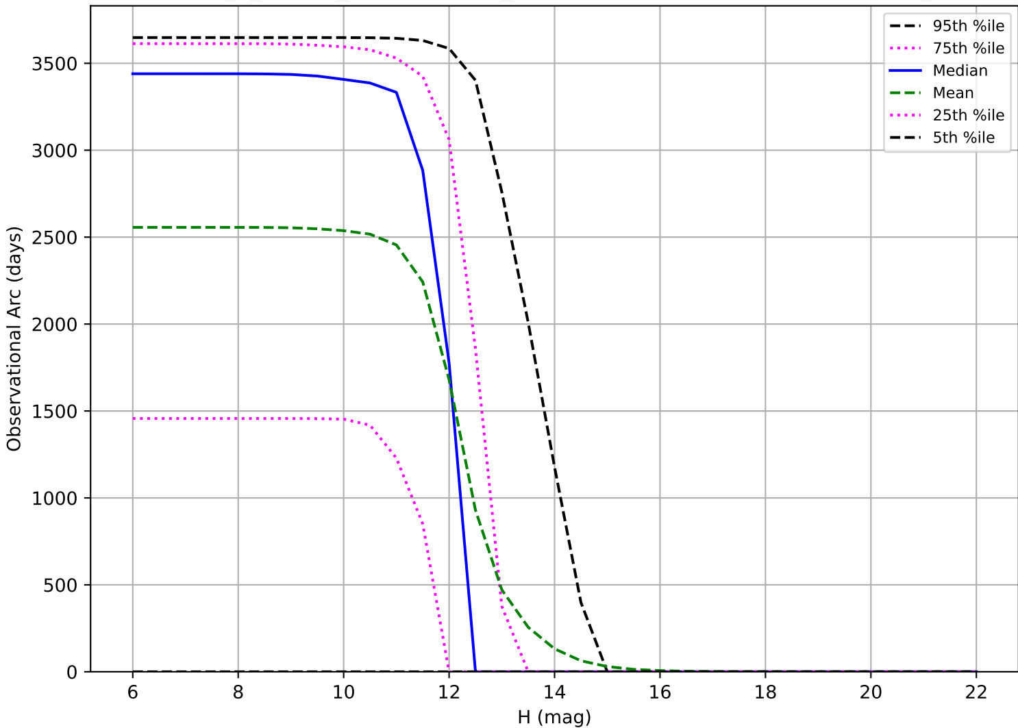
internal_u_expt30_nscale0.9v3.4_10yrs: Observational Arc Length OCC_r20
