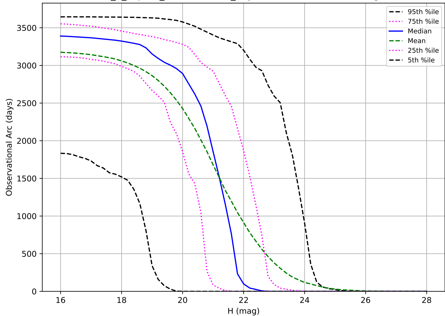
internal_u_expt30_nscale0.9v3.4_10yrs: Observational Arc Length NEO
