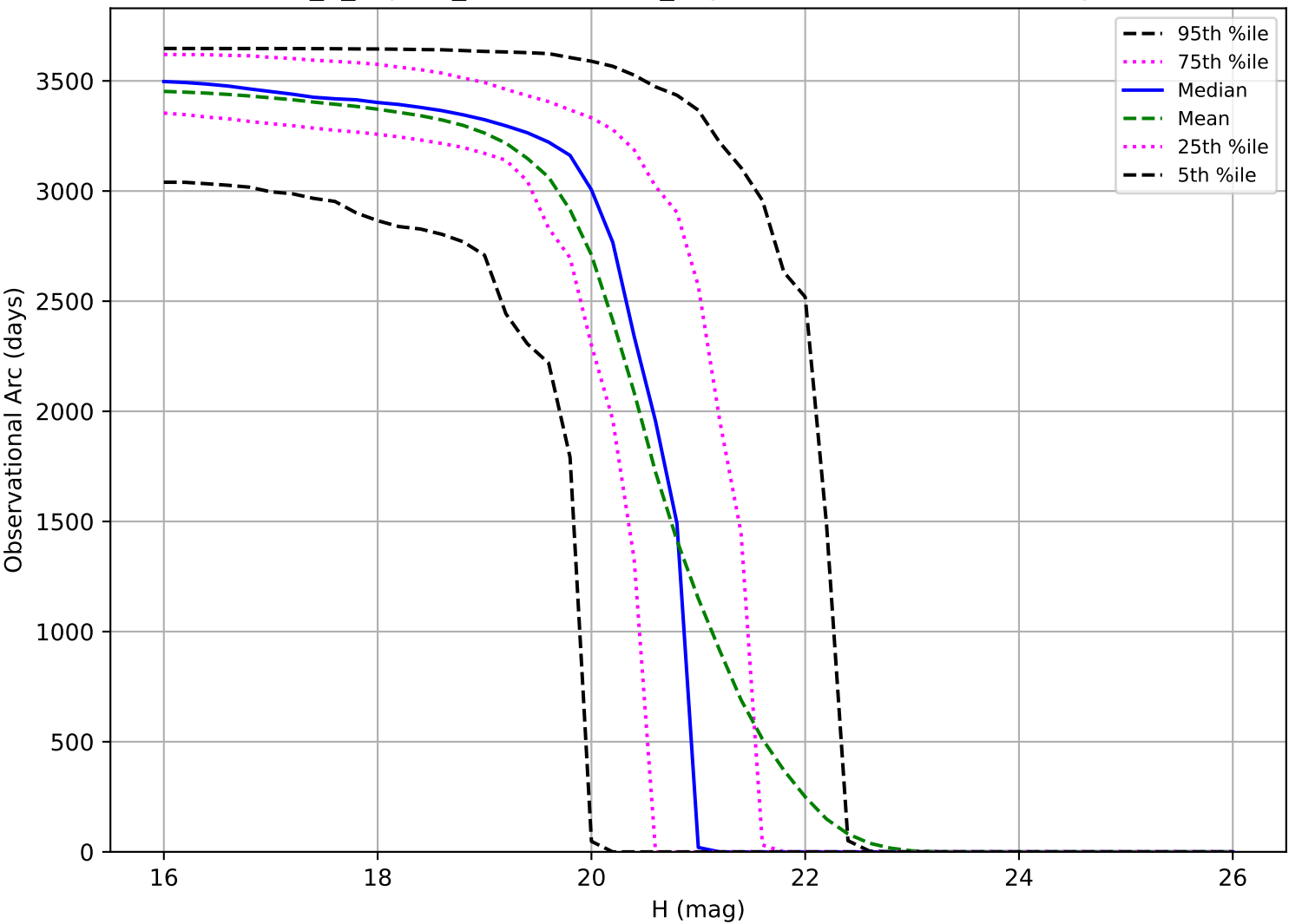
internal_u_expt30_nscale0.9v3.4_10yrs: Observational Arc Length MBA
