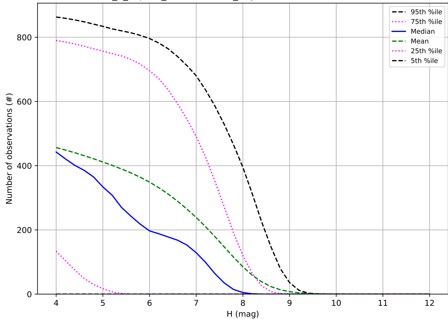
internal_u_expt30_nscale0.9v3.4_10yrs: Number of observations TNO
