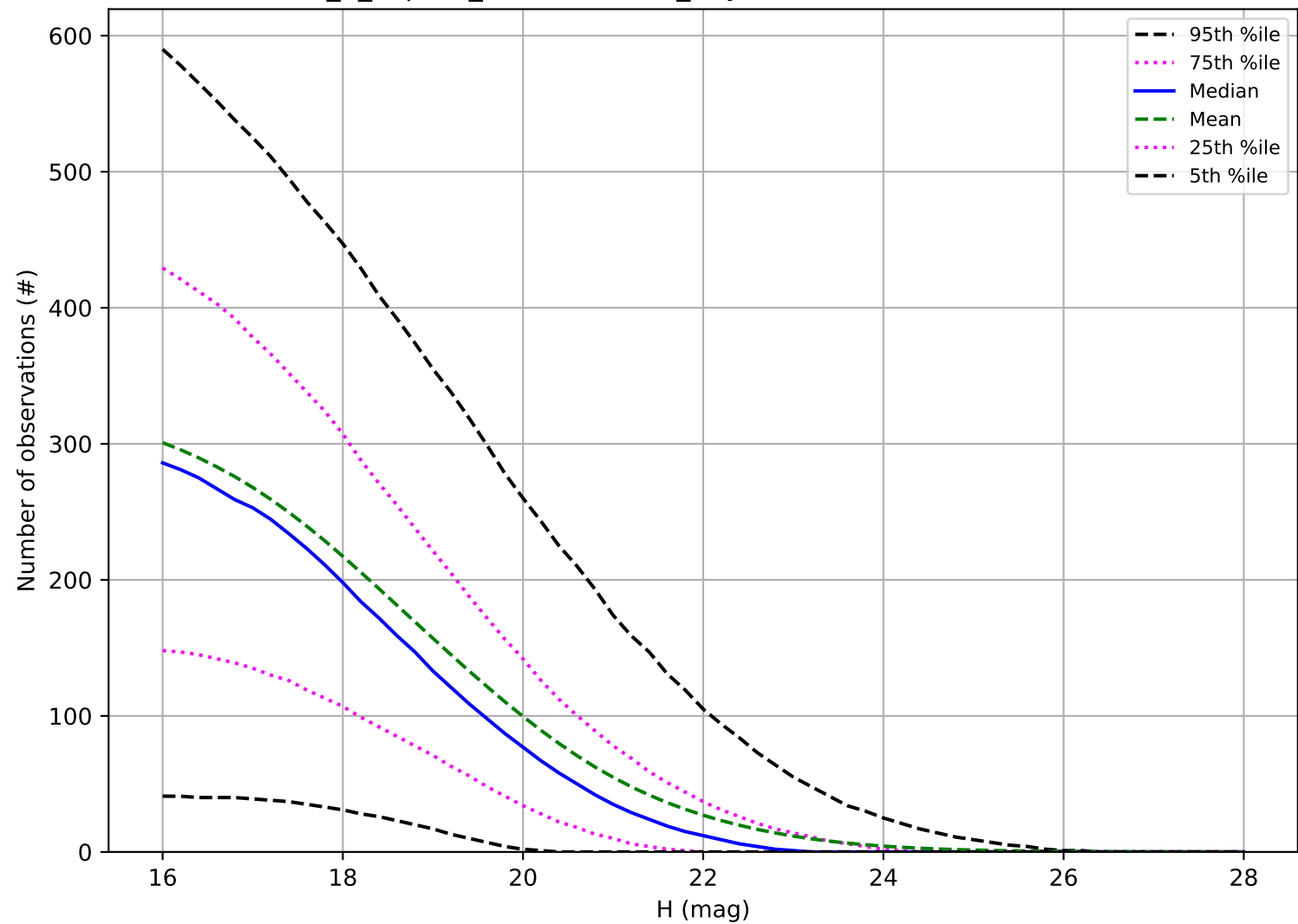
internal_u_expt30_nscale0.9v3.4_10yrs: Number of observations PHA
