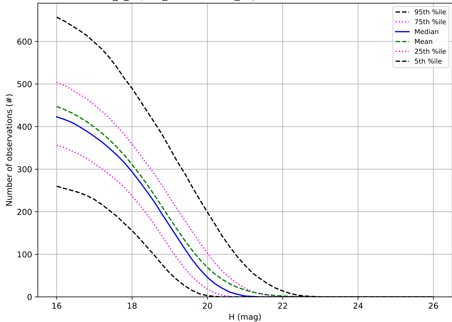
internal_u_expt30_nscale0.9v3.4_10yrs: Number of observations MBA
