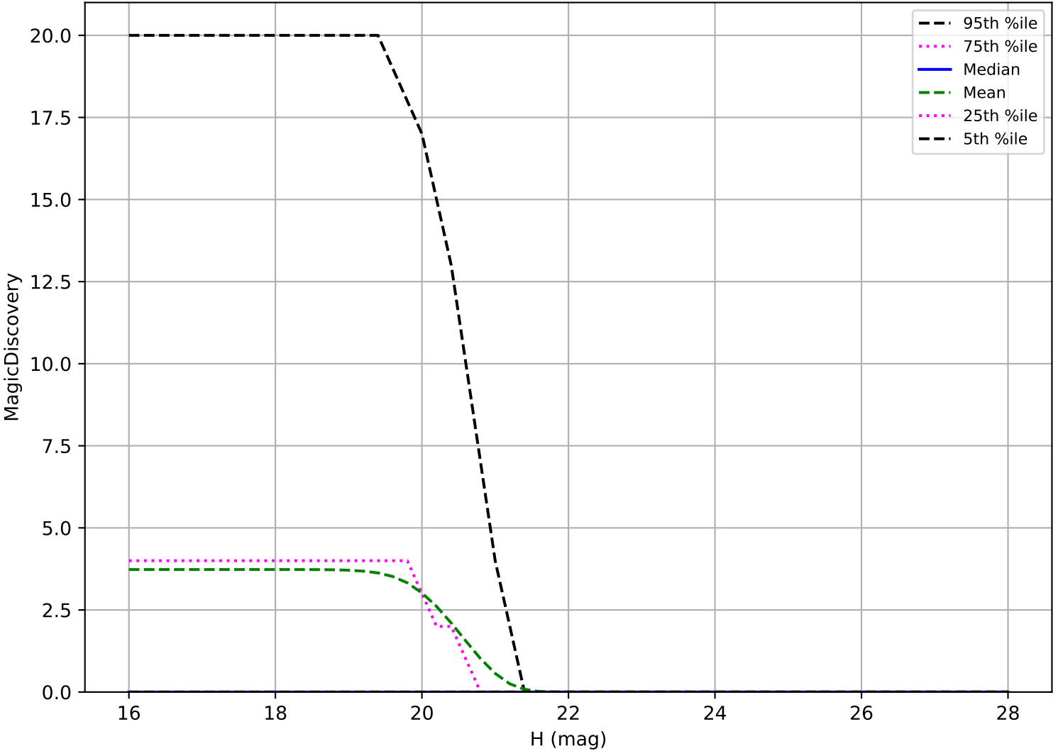
internal_u_expt30_nscale0.9v3.4_10yrs: Vatira 6 detections in 60 nights detection loss
