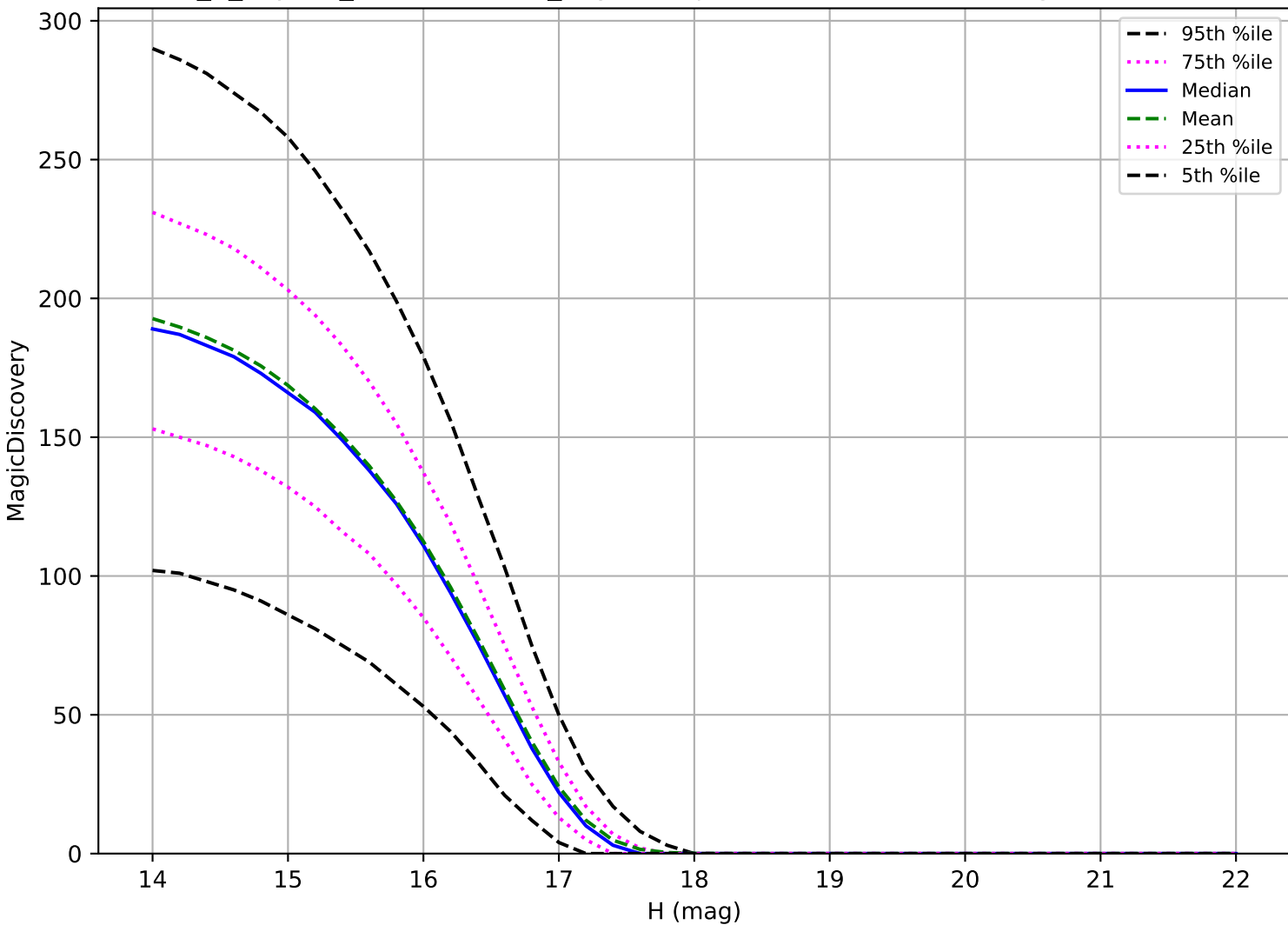
internal_u_expt30_nscale0.9v3.4_10yrs: Trojan 6 detections in 60 nights detection loss
