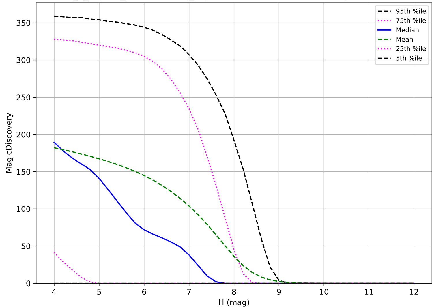
internal_u_expt30_nscale0.9v3.4_10yrs: TNO 6 detections in 60 nights detection loss
