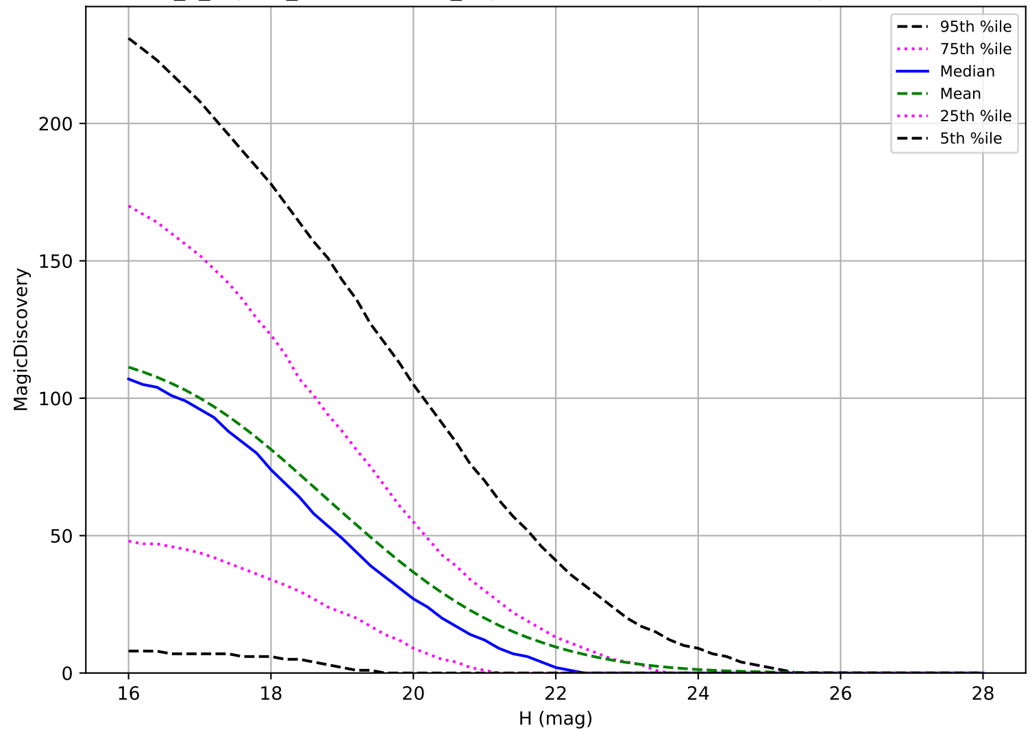
internal_u_expt30_nscale0.9v3.4_10yrs: PHA 6 detections in 60 nights detection loss
