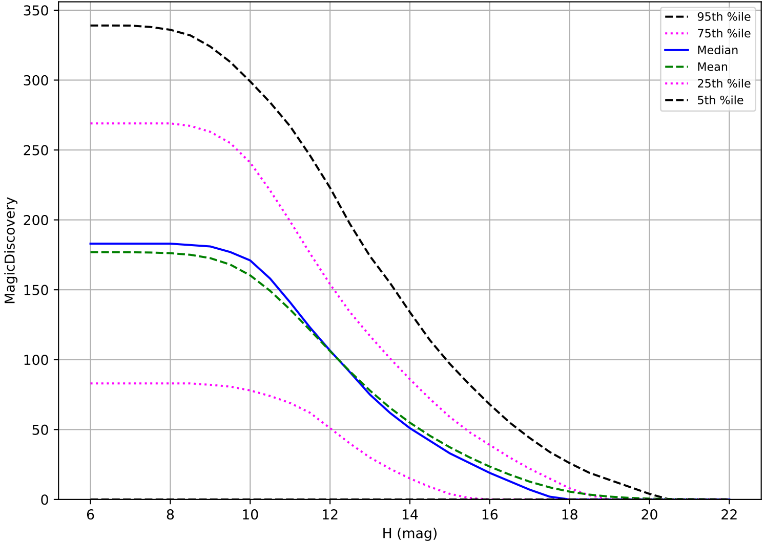
internal_u_expt30_nscale0.9v3.4_10yrs: OCC_r5 6 detections in 60 nights detection loss
