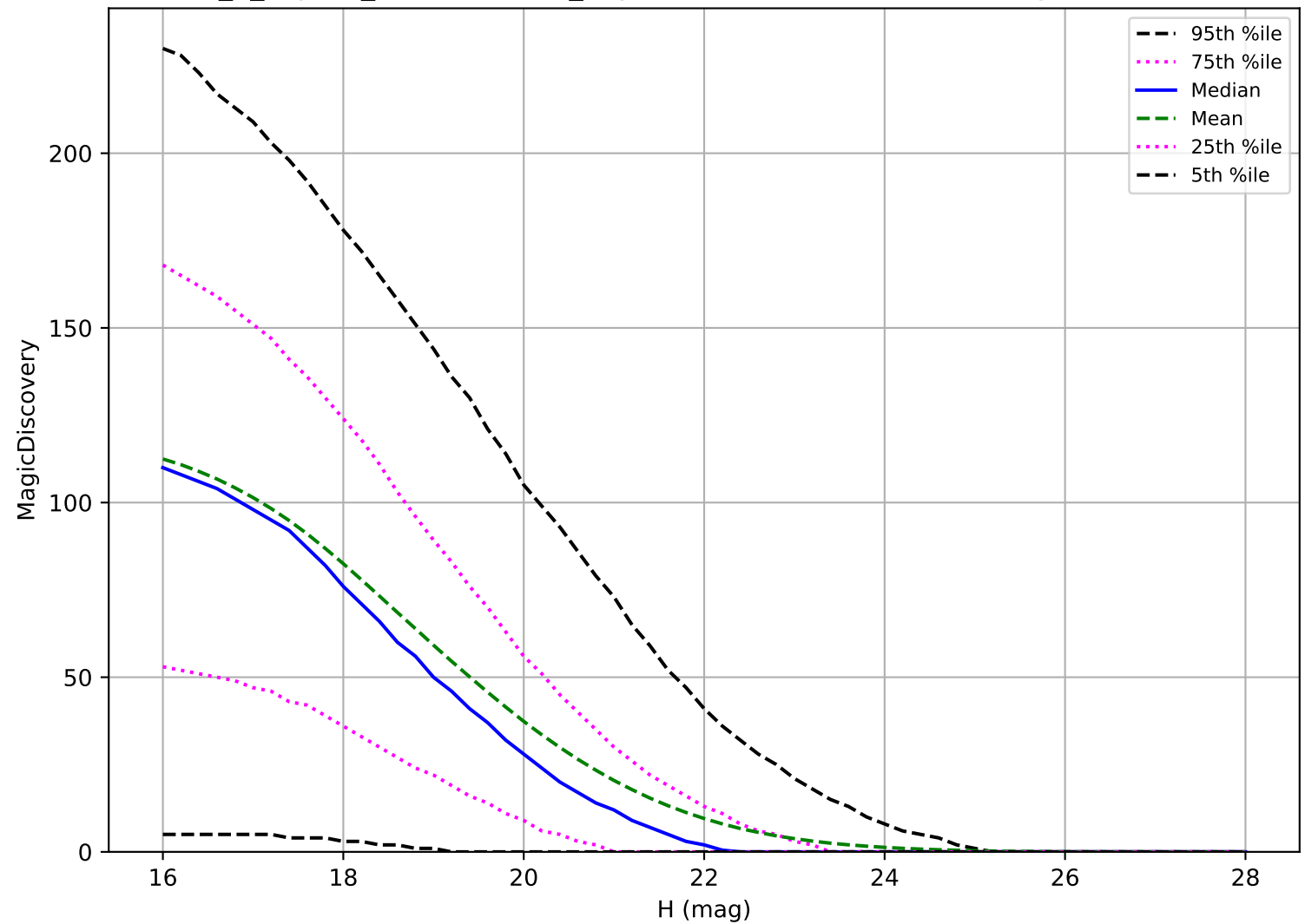
internal_u_expt30_nscale0.9v3.4_10yrs: NEO 6 detections in 60 nights detection loss
