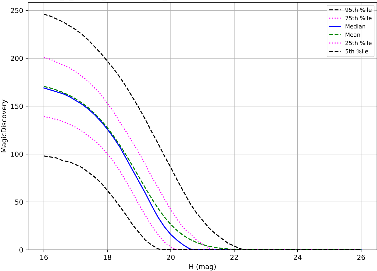
internal_u_expt30_nscale0.9v3.4_10yrs: MBA 6 detections in 60 nights detection loss
