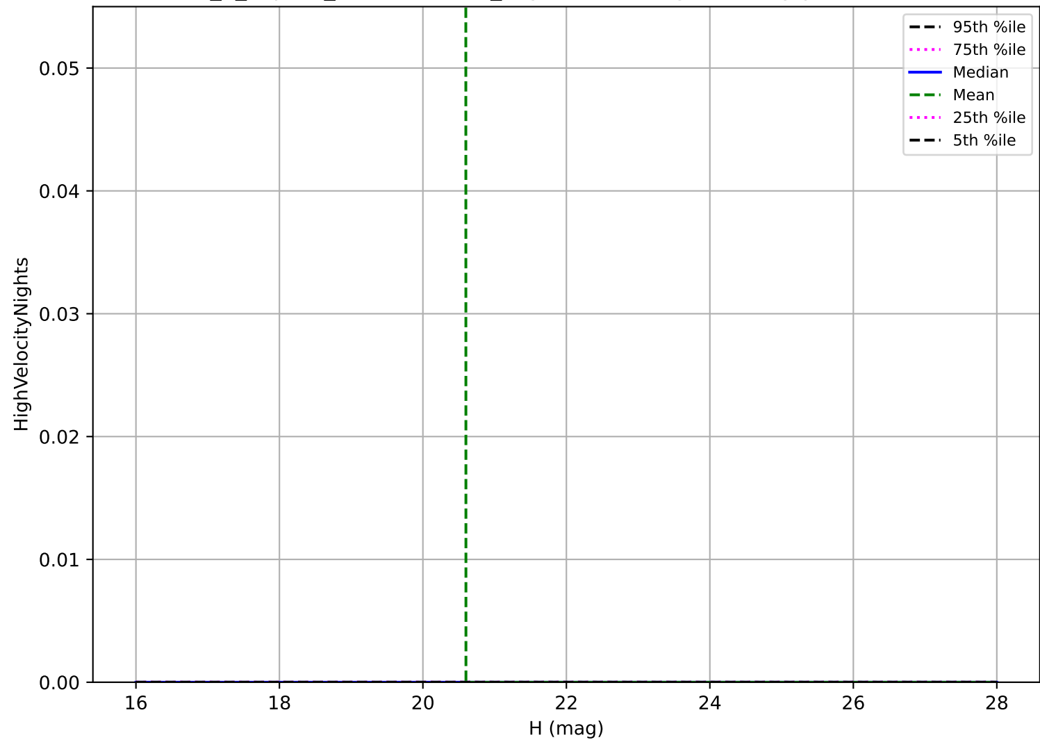
internal_u_expt30_nscale0.9v3.4_10yrs: Vatira High velocity pair detection loss
