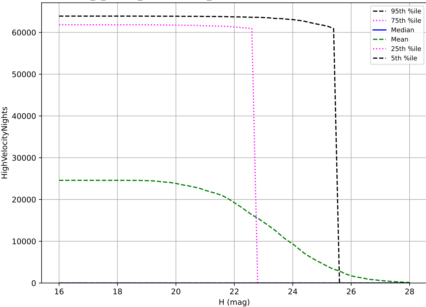
internal_u_expt30_nscale0.9v3.4_10yrs: PHA High velocity pair detection loss
