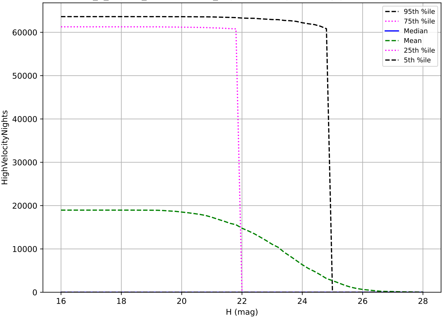
internal_u_expt30_nscale0.9v3.4_10yrs: NEO High velocity pair detection loss
