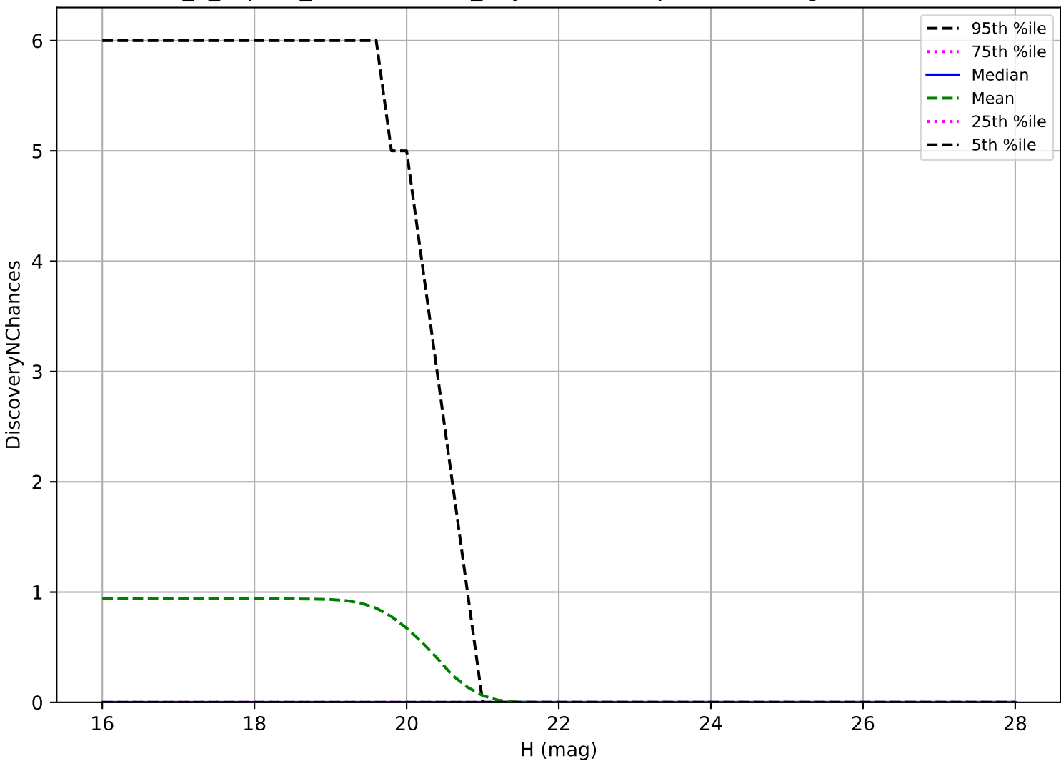
internal_u_expt30_nscale0.9v3.4_10yrs: Vatira 3 pairs in 15 nights detection loss
