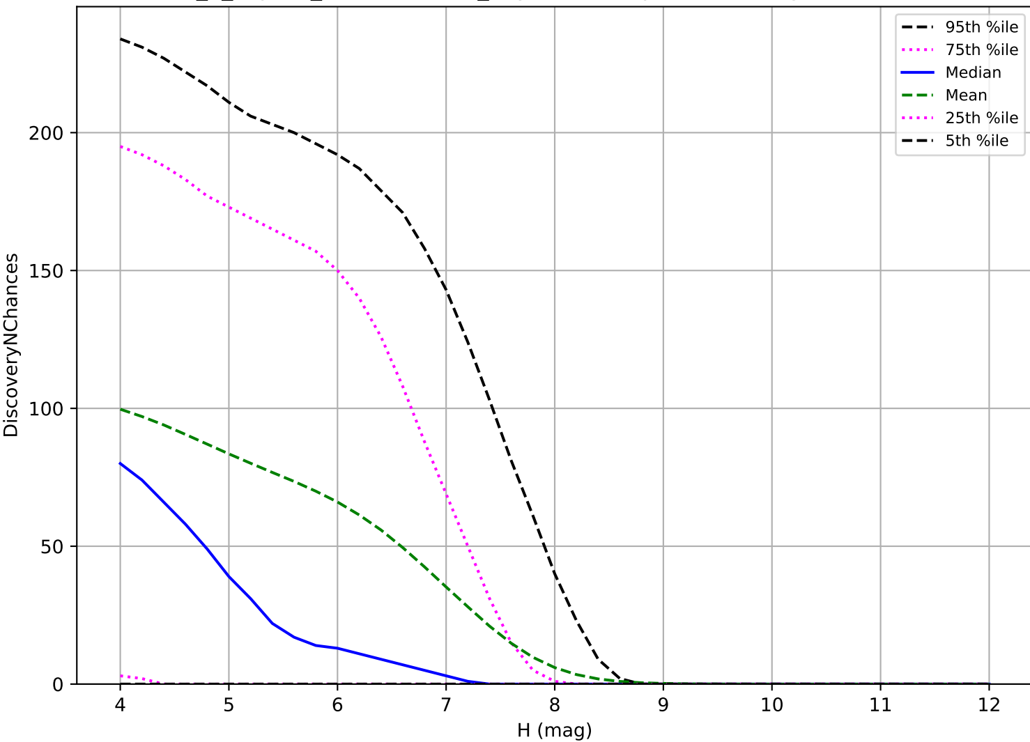
internal_u_expt30_nscale0.9v3.4_10yrs: TNO 3 pairs in 15 nights detection loss
