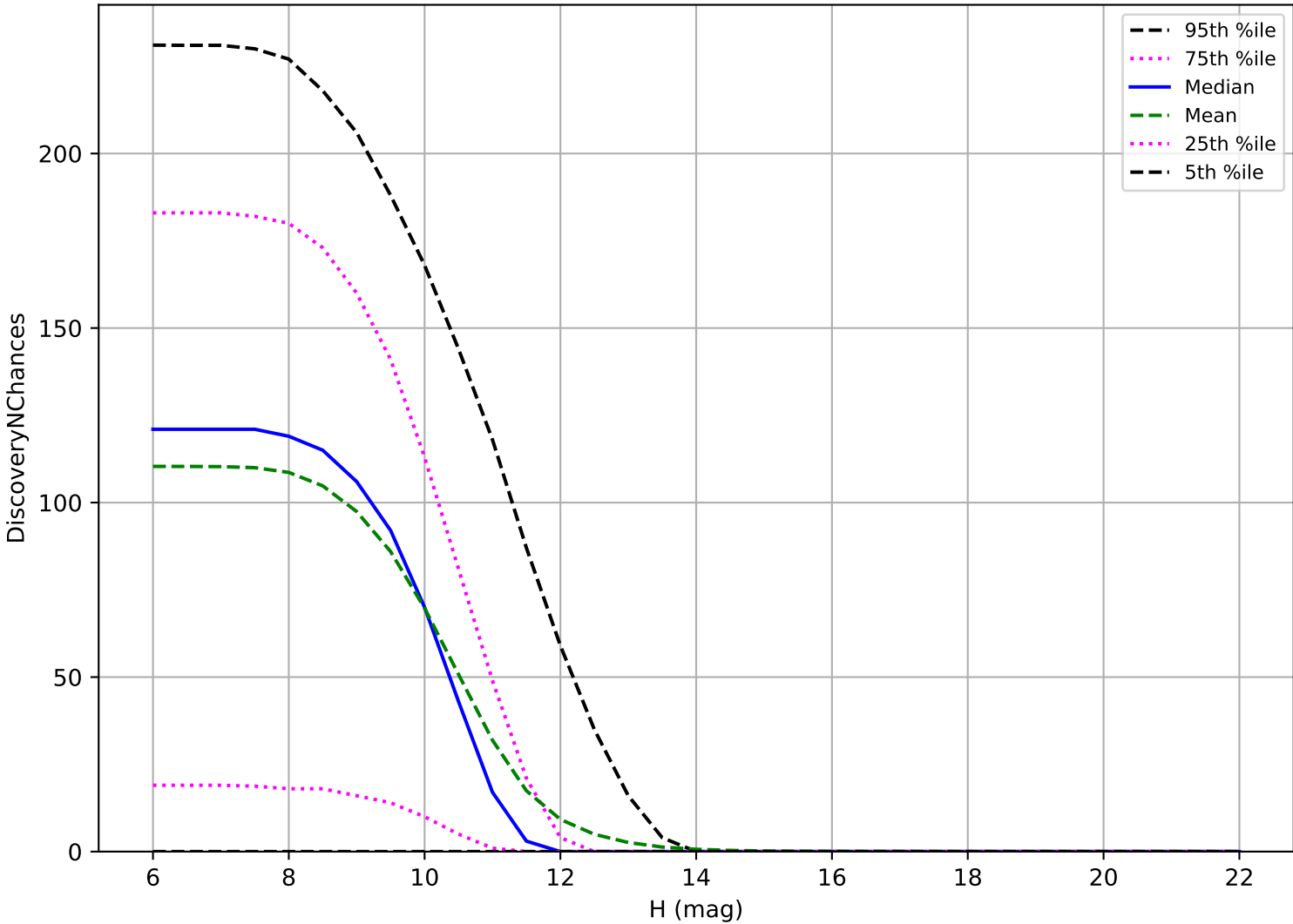
internal_u_expt30_nscale0.9v3.4_10yrs: OCC_r20 3 pairs in 15 nights detection loss
