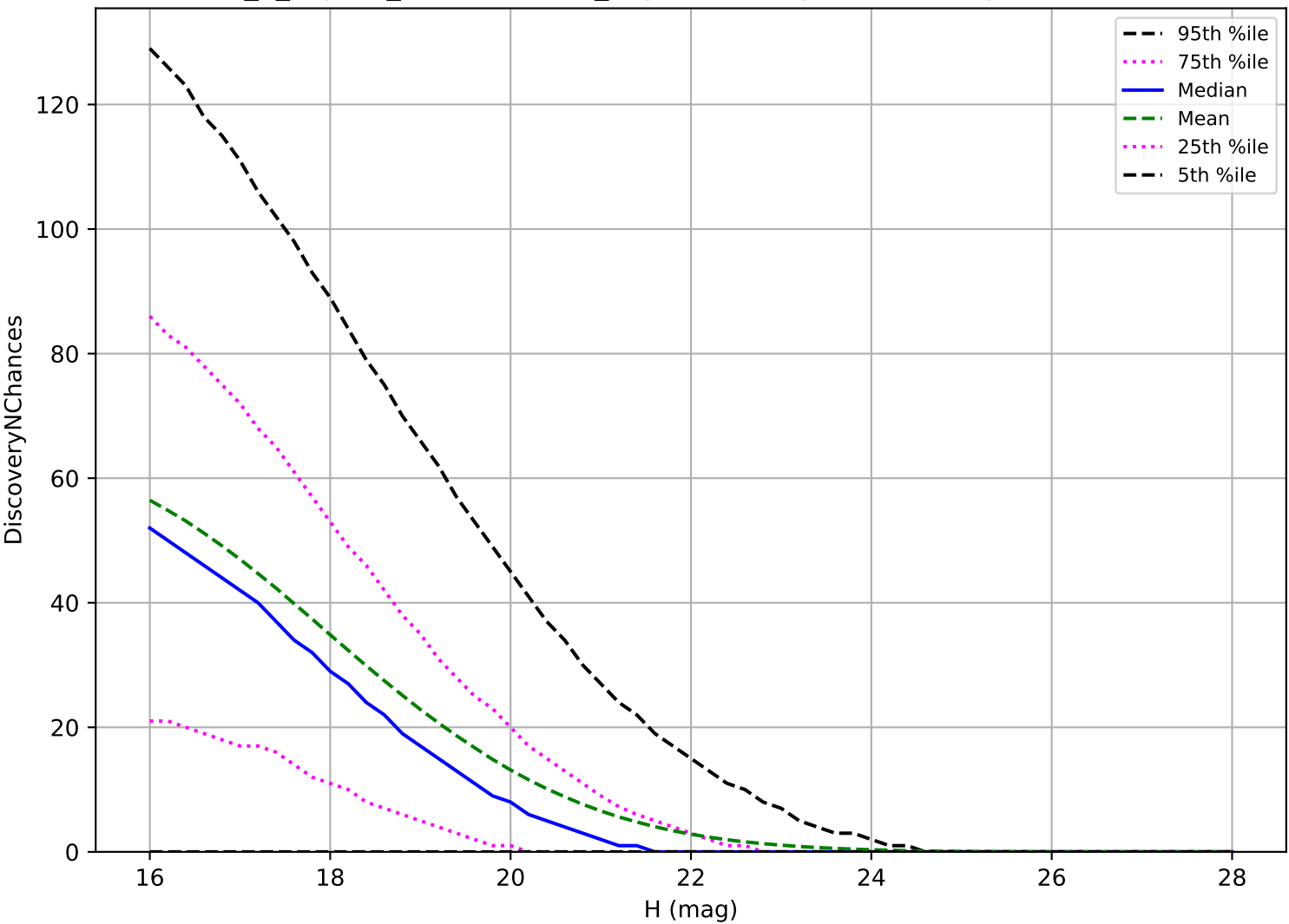
internal_u_expt30_nscale0.9v3.4_10yrs: NEO 3 pairs in 15 nights detection loss
