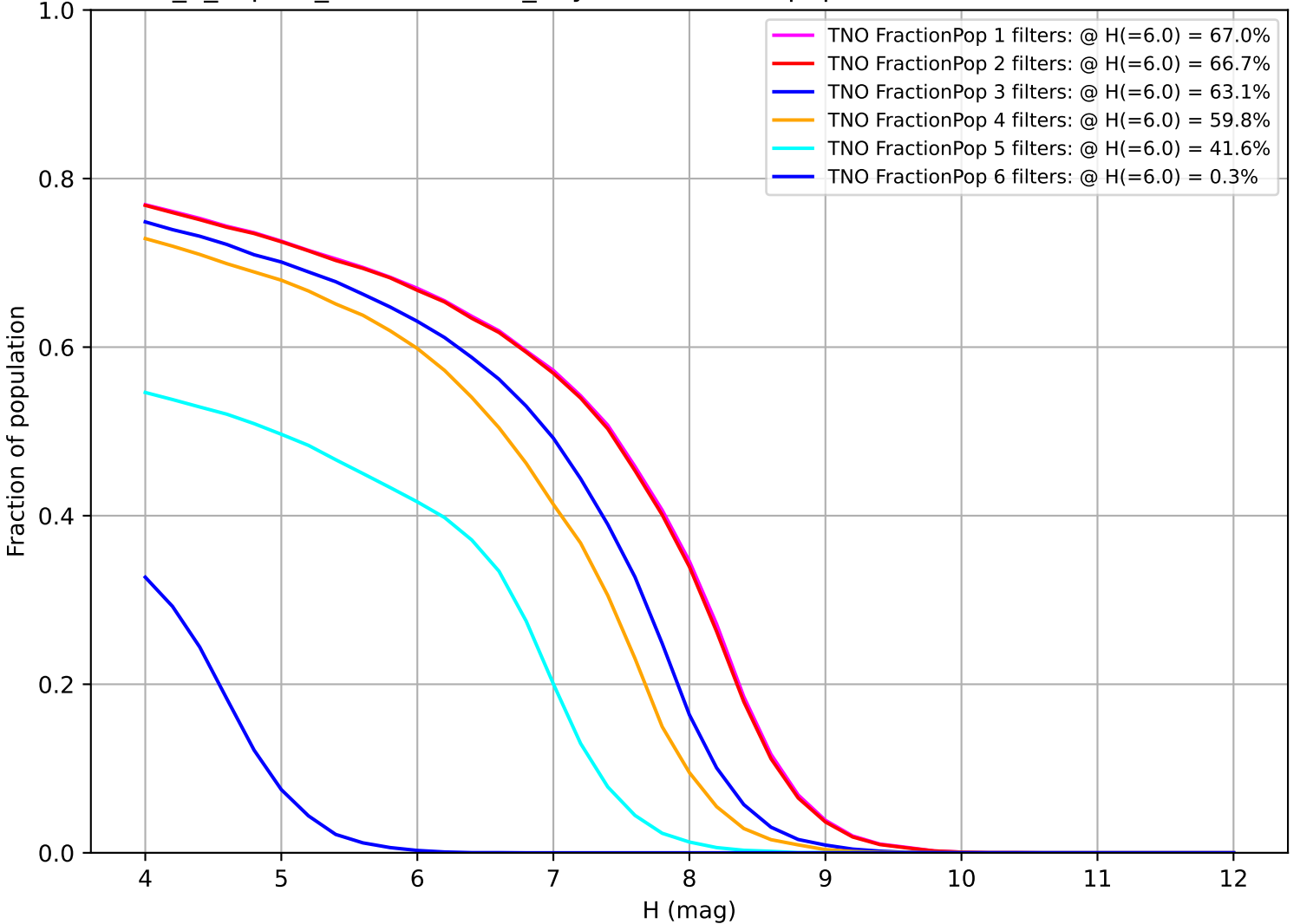
internal_u_expt30_nscale0.9v3.4_10yrs: Fraction of population with colors in X filters TNO
